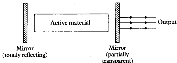
14.3 Schematic diagram of a laser in which the active material is confined between plane parallel mirrors.
